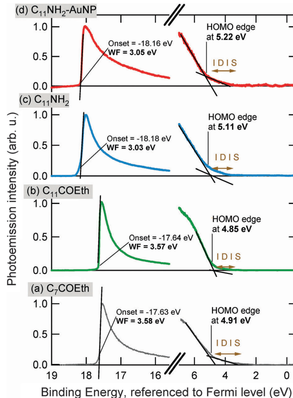
Fig. 4 Secondary electron (SE) edges (left part of the spectra) and valence UP Spectra (right spectra) of (a) C_7 -COEth, (b) C_{11} -COEth, (c) C_{11} - NH_2 , and (d) C_{11} - NH_2 -AuNP. The cutoffs of the SE curves are indicated by the vertical bars and are used to calculate the work functions of the different organic monolayers. The edges of the UP Spectra correspond to the highest occupied molecular orbital (HOMO).
